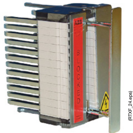
Figure 6: Block-plug handle, RTXF 24
