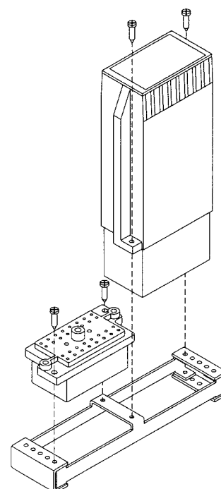
Figure 2: The assembly of RTXP 8 and terminal base RX 1 with the 4U adapter
